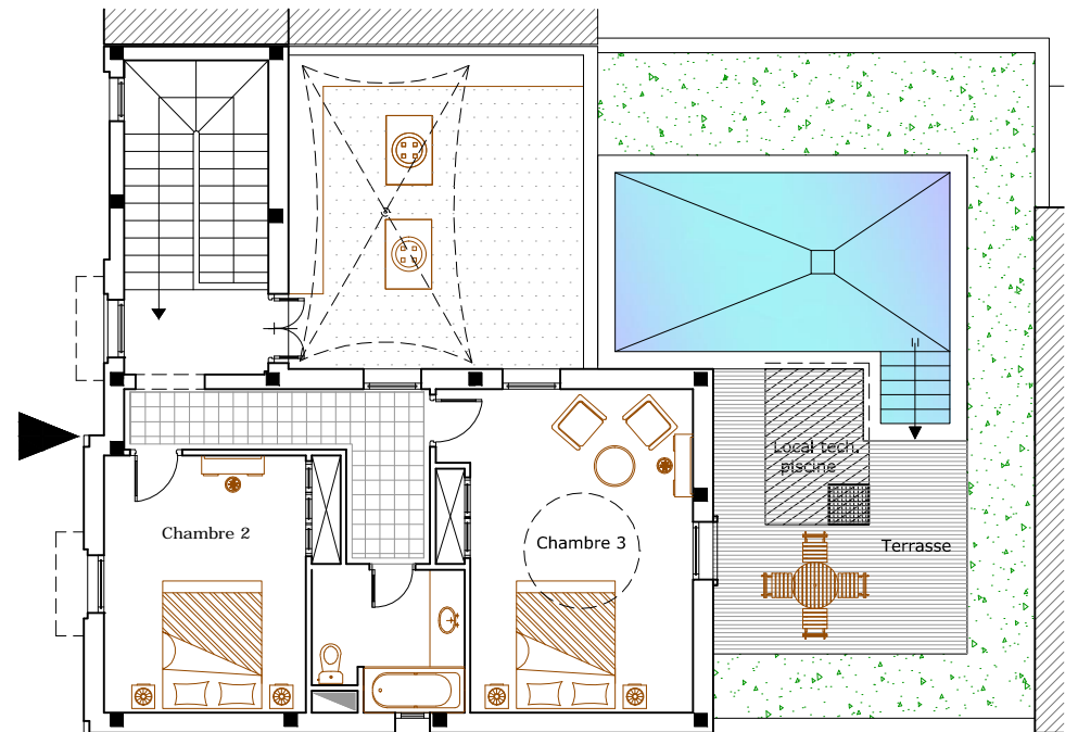
Plan R+1
